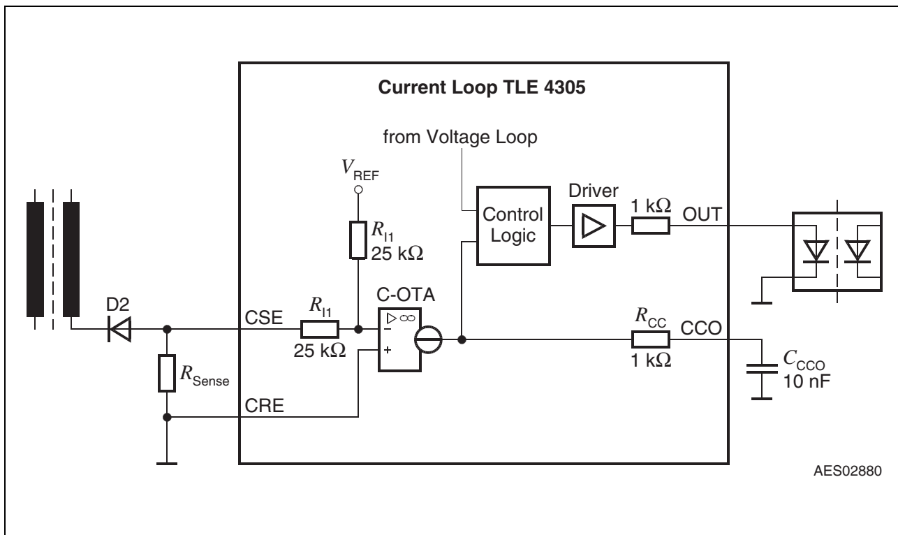
Figure 7 Current Control Loop
